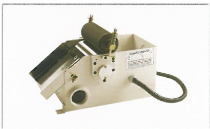
13. Magnetic coolant separator
