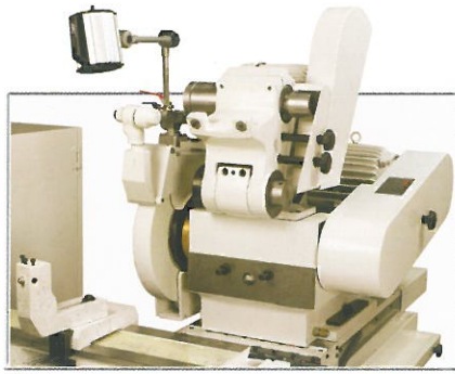
1. Internal grinding attachment (including one spindle)
