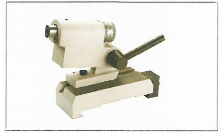
2. Diamond tool holder for internal and external grinding wheel dressing (upward open type)
